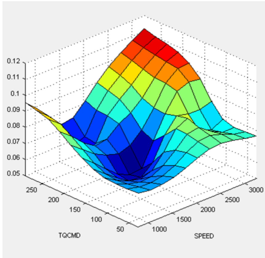
Pilot Fuel Mass Fraction Table
