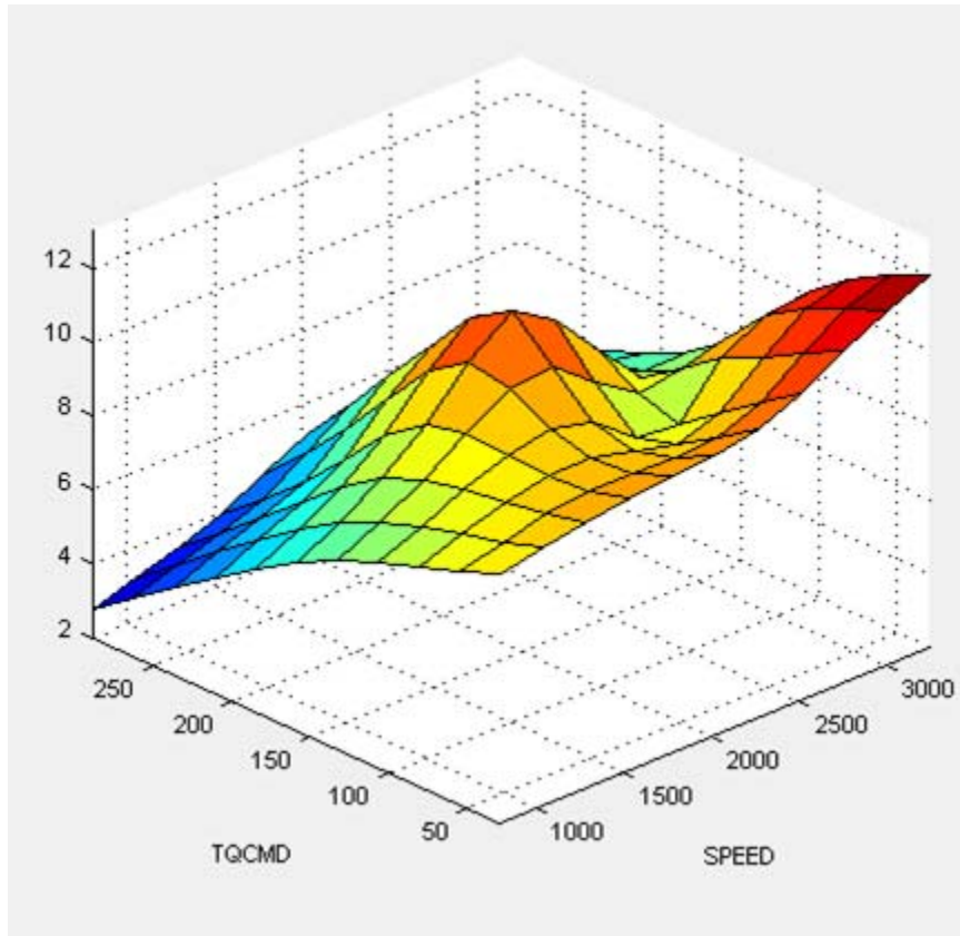
Pilot Injection Timing (Pilot SOI Delta) Table
