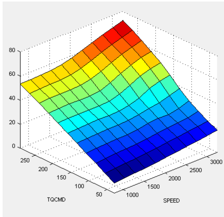
Total Injected Fuel Mass Table
