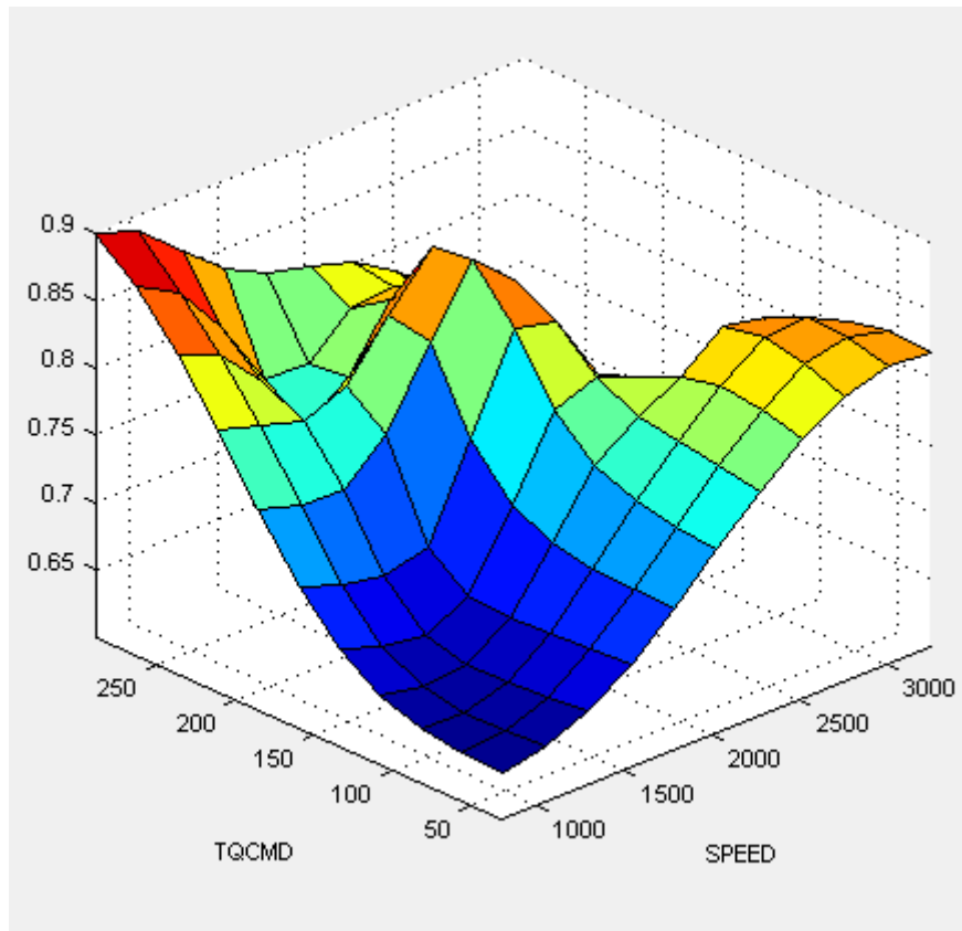
Variable-Geometry Turbo (VGT) Position Table
