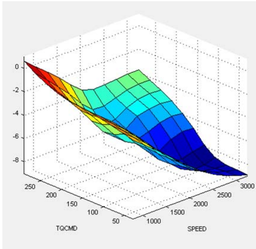
Main Injection Timing (SOI) Table
