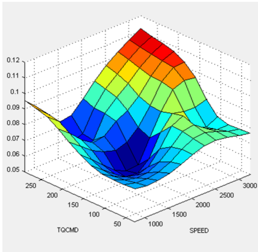
Pilot Fuel Mass Fraction Table
