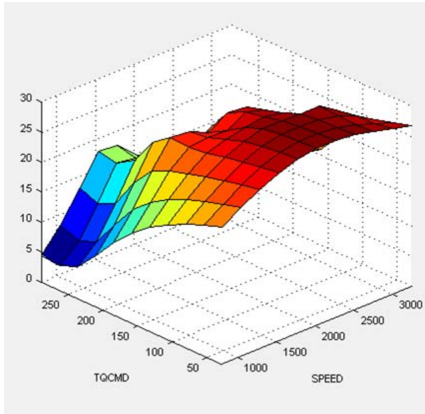
Fuel Pressure Delta Table
