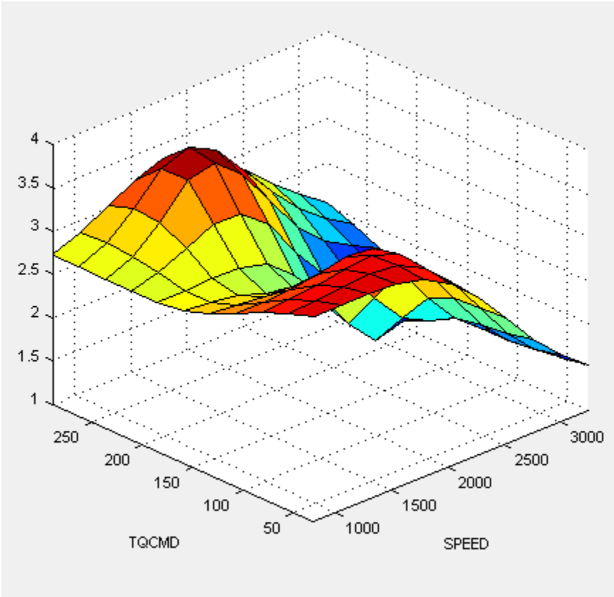
Exhaust Gas Recirculation (EGR) Valve Position Table
